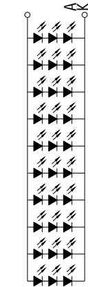
Backlight LED Circuit Circuit Diagram(LED SMT 3*10=30 PCS), Color: WHITE VF=8.4-10.5V, I f=200mA Brightness 500cd/m2(TYP)
